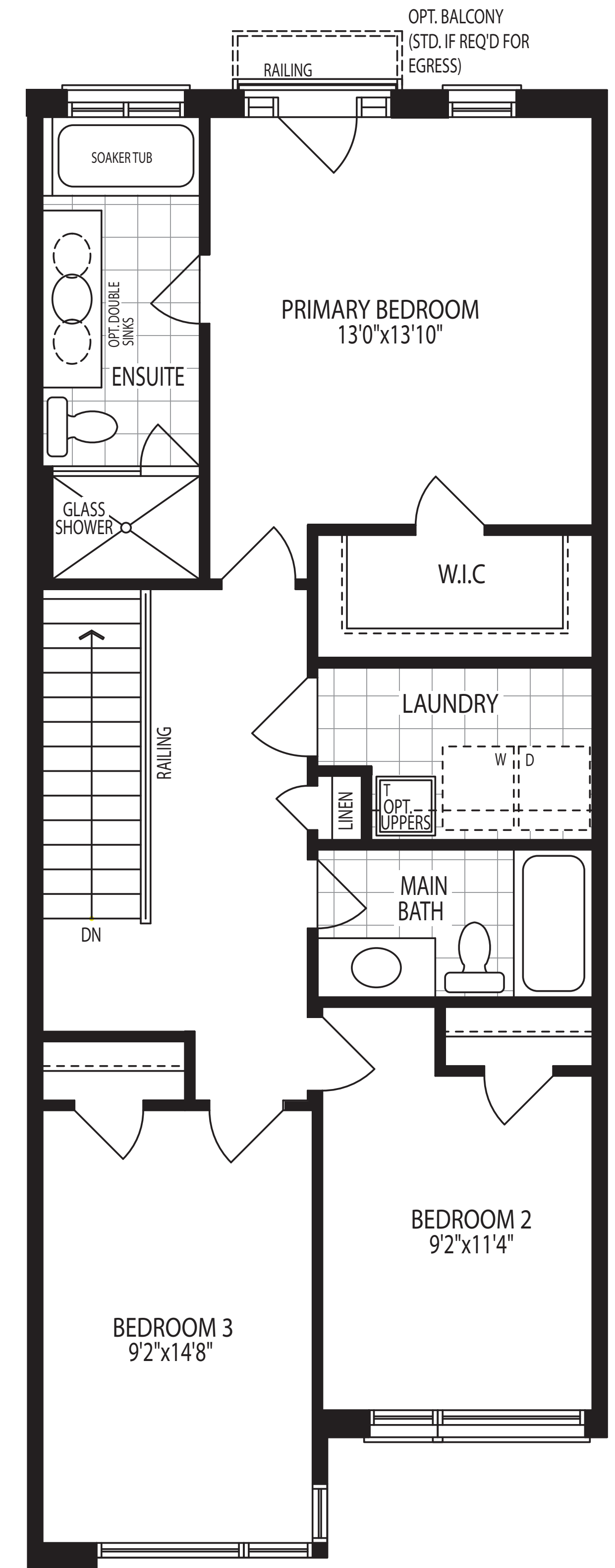
UPPER FLOOR PLAN ELEV. D
