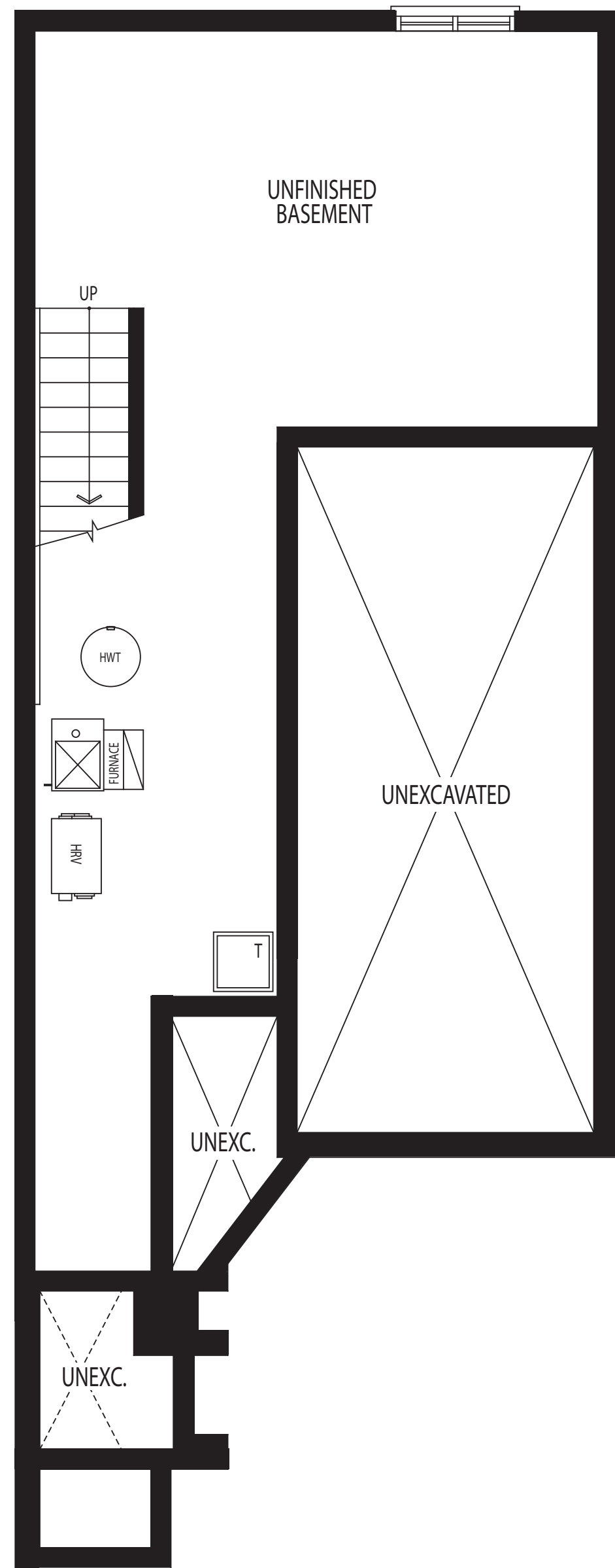
BASEMENT PLAN ELEV. D & E
