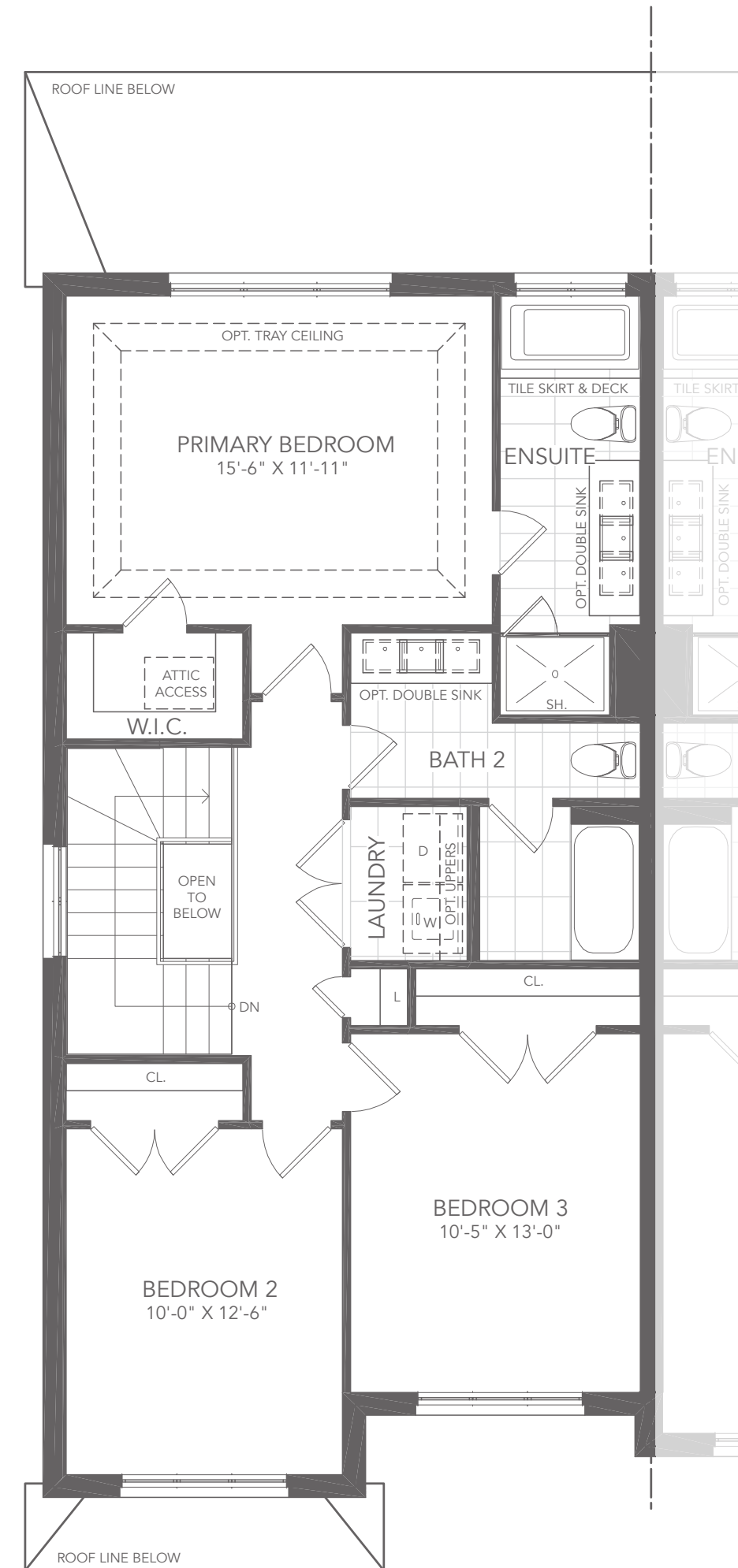
SECOND FLOOR PLAN A
