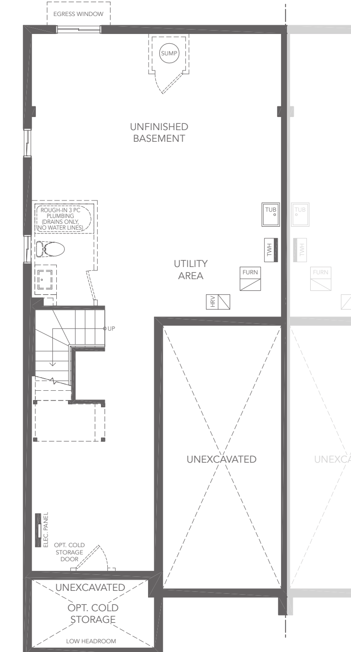
BASEMENT PLAN A
