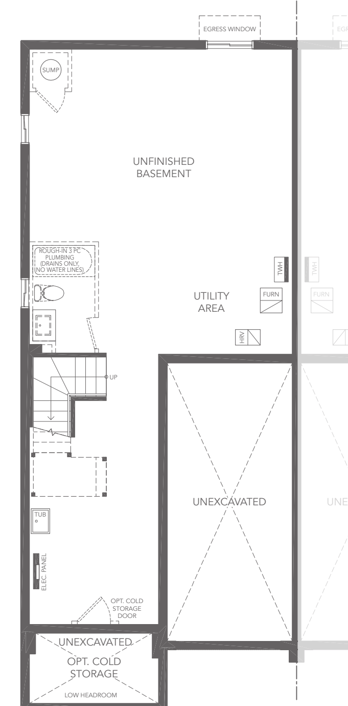
BASEMENT PLAN A
