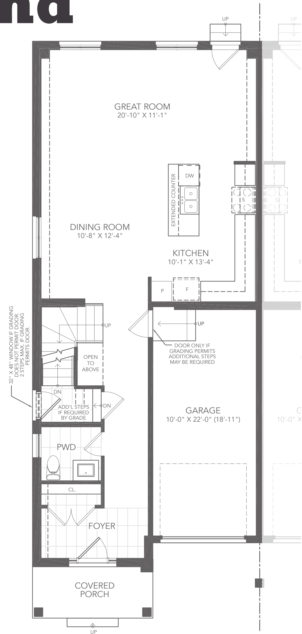
GROUND FLOOR PLAN A
