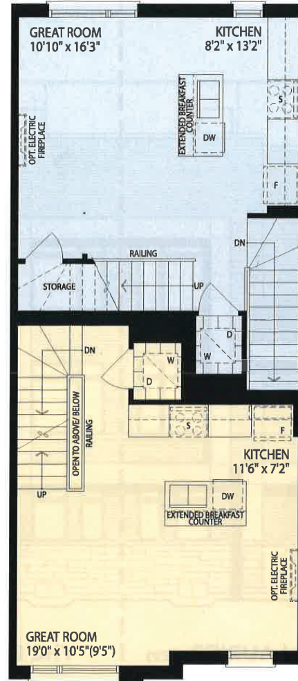
SUITE 1 MAIN FLOOR ELEV. 'B'
